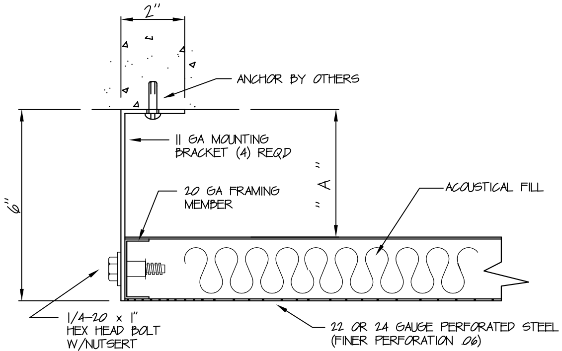
LONGITUDINAL SECTION OFFSET MOUNT
